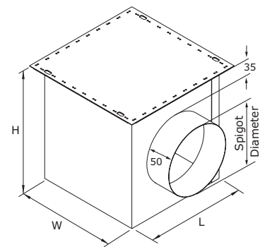
PBG - Side entry grille plenum box
