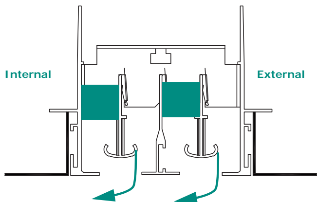
Figure 2- Internal air flow
