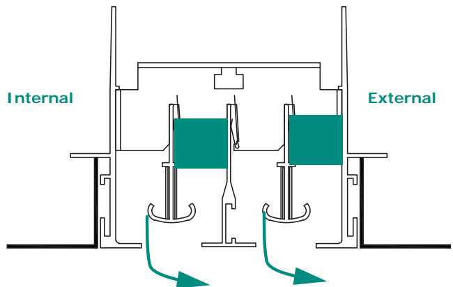
Figure 3- External air flow
