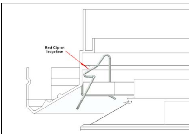
Figure 10a: Rest Bunny Clip on Ledge
