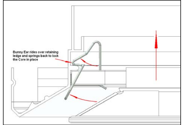
Figure 11a: Clip springs into position
