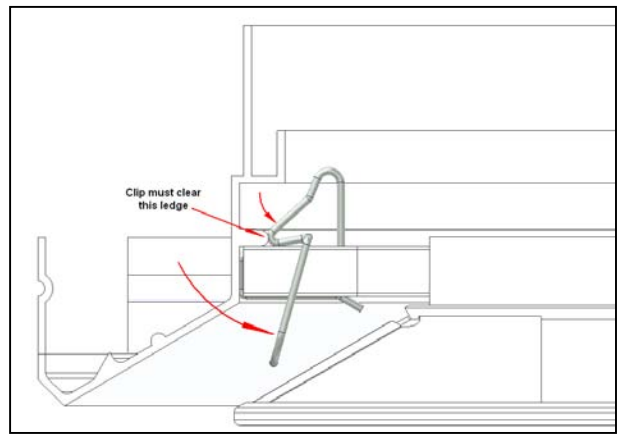
Figure 3: Push Clip inwards to release
