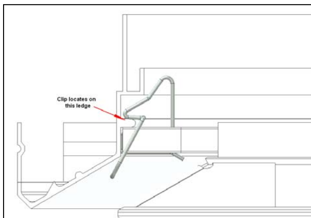
Figure 2a: Bunny Clip Detail
