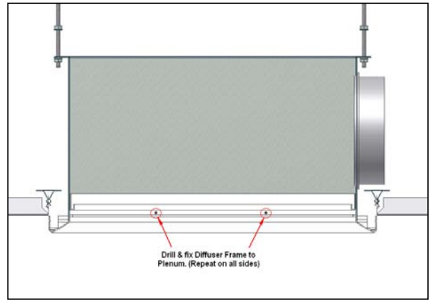
Figure 7: Drill & fix Frame & Plenum
