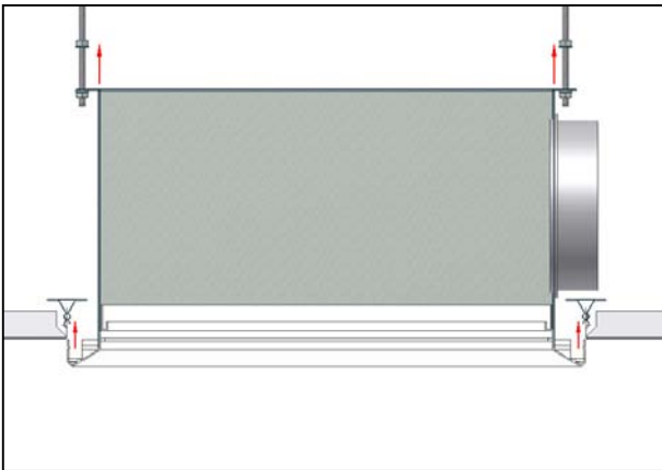
Figure 8: Raise the Plenum & Diffuser
