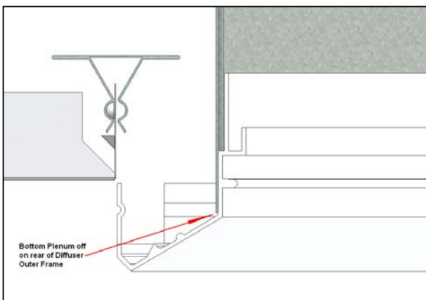
Figure 6a: Butt Plenum on Frame
