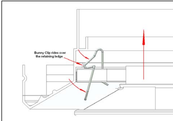
Figure 11: Clip rides over ledge
