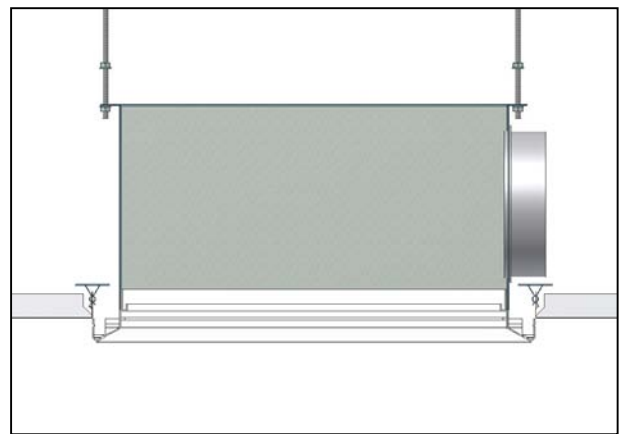
Figure 6: Locate Diffuser in Plenum
